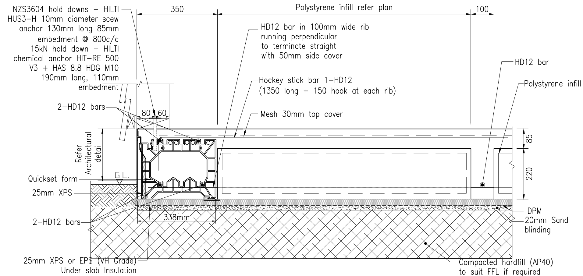
TIMBER WEATHER BOARD PERIMETER DETAIL
