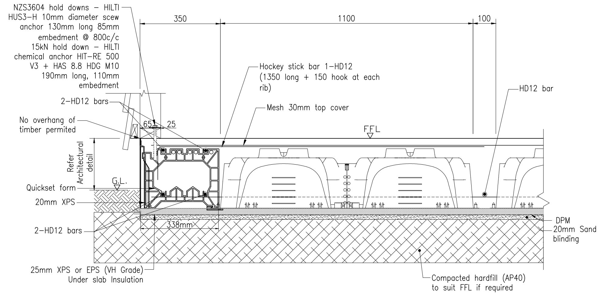
TIMBER WEATHER BOARD QPod PERIMETER DETAIL
