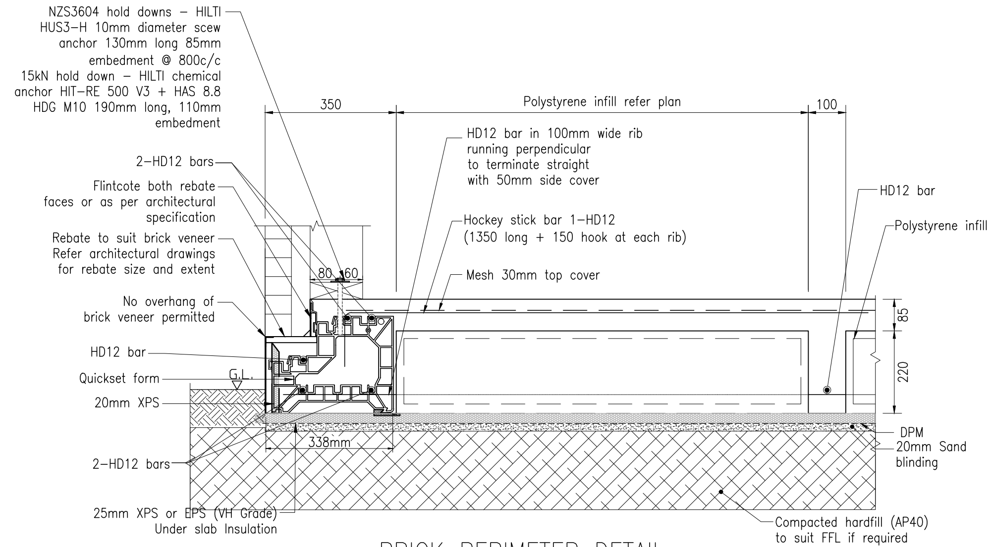
BRICK PERIMETER DETAIL
