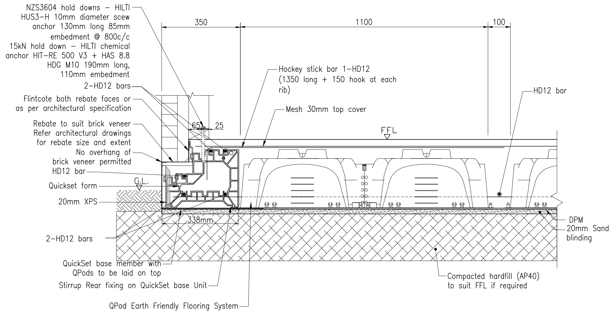
BRICK QPod PERIMETER DETAIL WITH NO UNDERSLAB INSULATION
